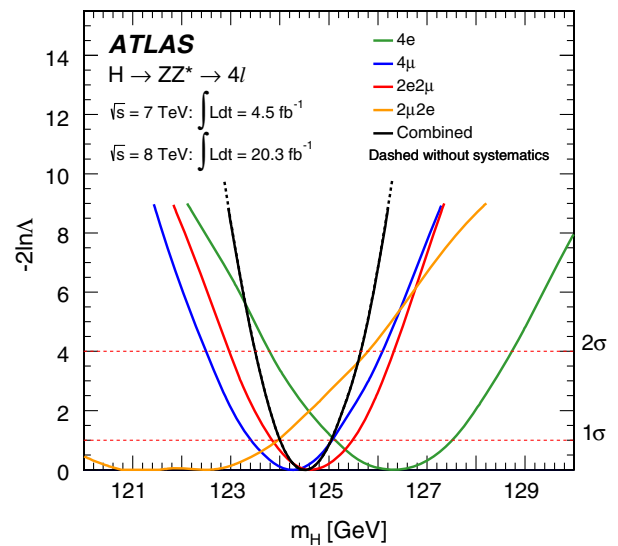
FIG. 7 (color online). The profile likelihood as a function of m_H for the combination of all H \rightarrow ZZ^* \rightarrow 4\ell channels and for the individual channels for the combined 7 TeV and 8 TeV data samples. The combined result is shown both with (solid line) and without (dashed line) systematic uncertainties, and the two results are almost indistinguishable.
