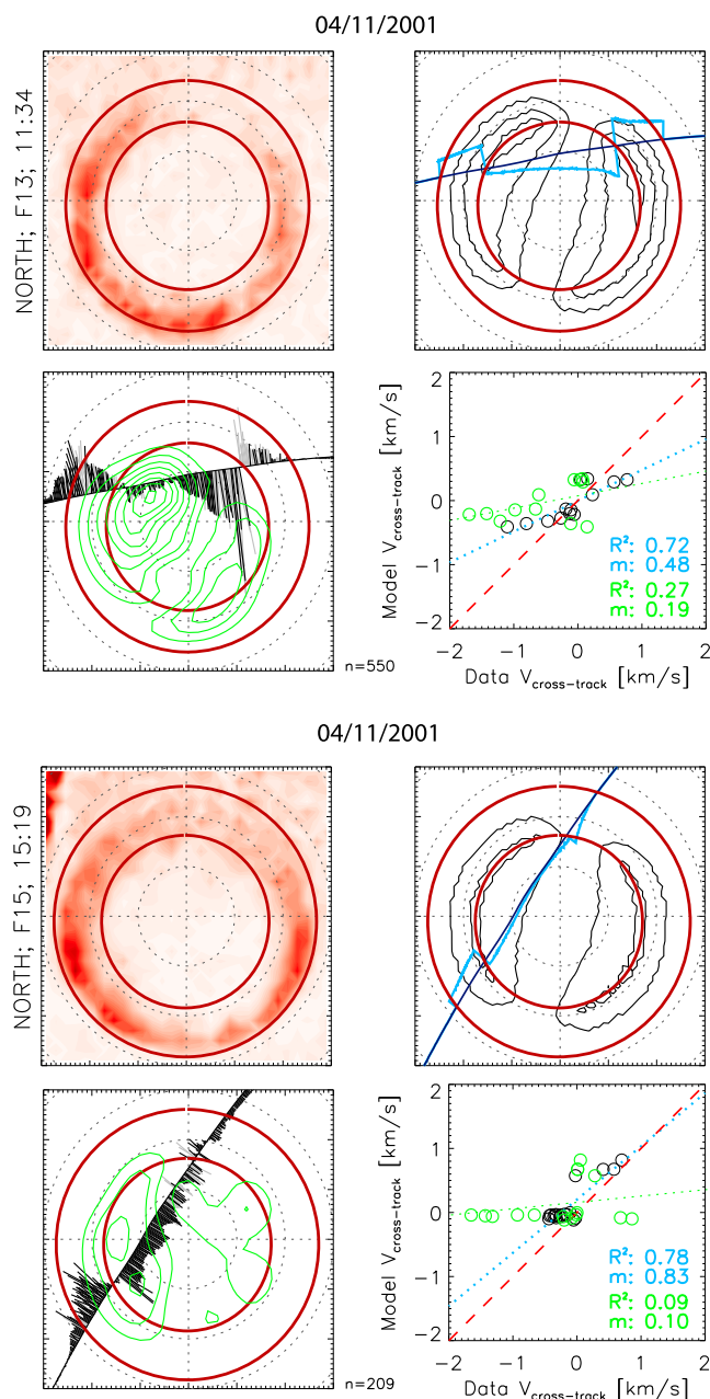
Figure 3. Two individual DMSP orbits for 4 November 2001, showing the IMAGE data with (top left) fitted circles (colored map); (top right) the model equipotentials (black) and cross-track velocities (blue); (bottom right) DMSP cross-track velocities and SuperDARN equipotentials and a scatterplot of the cross-track velocities. The potentials are spaced at regular intervals of 6 kV. Each orbit is centered on the geomagnetic poles, and the concentric circles in dashed grey are spaced at 10° of geomagnetic latitudes each. The green data in the scatterplots show the cross-track velocities derived from SuperDARN. The red dashed line shows the line of unity, and the dotted lines show the lines of best fit (green = SuperDARN and blue = DMSP).
