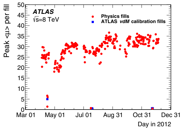
Fig. 12 History of the peak bunch-averaged pile-up parameter \langle \mu \rangle during 2012, restricted to stable-beam periods
