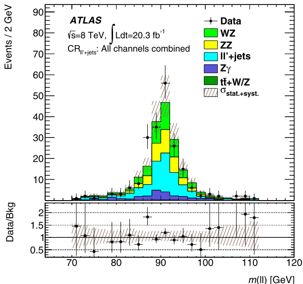
Fig. 2. Z candidate invariant mass distribution in the \ell\ell' + \text{jets} background control region ( CR_{\ell\ell'+\text{jets}} ). The uncertainty bands upon the expected background include both the statistical and systematic uncertainties in the MC simulation and the fake-background estimation added in quadrature.
