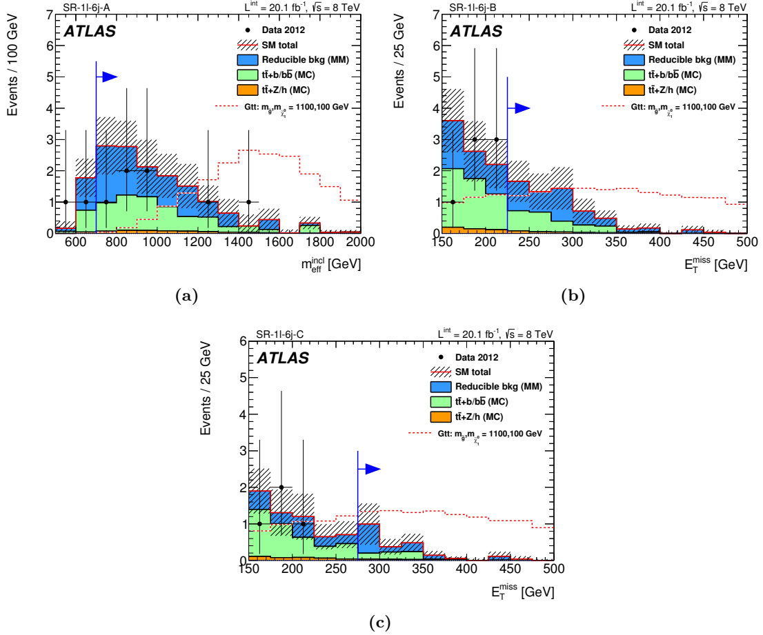
Figure 10. The (a) m_{\text{eff}}^{\text{incl}} and (b)-(c) E_T^{\text{miss}} distribution observed in data for SR-1l-6j-A, SR-1l-6j-B and SR-1l-6j-C, respectively, after all requirements applied but the one indicated by the arrow, together with the background prediction. The shaded bands include all experimental systematic uncertainties on the background prediction. The prediction for one signal point from the Gtt ( \tilde{g} \rightarrow t\bar{t}\tilde{\chi}_1^0 ) model is overlaid. The normalisation of the irreducible background t\bar{t} + b/b\bar{b} is as predicted by its theoretical cross-section scaled to the same luminosity as the data, prior to the fit in the control region.
