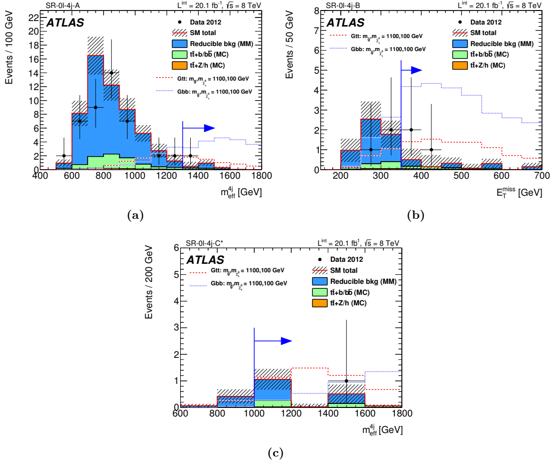
Figure 8. The (a)-(c) m_{\text{eff}}^{4j} and (b) E_T^{\text{miss}} distributions observed in data for SR-0 \ell -4j-A, SR-0 \ell -4j-B and SR-0 \ell -4j-C*, respectively, after all requirements applied but the one indicated by the arrow, together with the background prediction. The shaded bands include all experimental systematic uncertainties on the background prediction. The prediction for two signal points from the Gtt ( \tilde{g} \rightarrow t\bar{t}\tilde{\chi}_1^0 ) and Gbb ( \tilde{g} \rightarrow b\bar{b}\tilde{\chi}_1^0 ) models are overlaid. The normalisation of the irreducible background t\bar{t} + b\bar{b} is as predicted by its theoretical cross-section scaled to the same luminosity as the data, prior to the fit in the control region.
