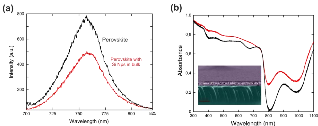
Figure 1 (a, b). (a) Comparison of PL spectra of perovskite film with embedded Si NPs in the bulk (red curve) and without it (black curve). (b) Absorbance spectra for the film with Si NPs (red) and without (black). Inset shows SEM image of perovskite film with Si NPs in the bulk.
