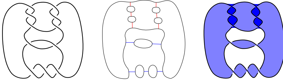
FIGURE 2. From left to right: An example link diagram, the graph \mathbb{G}_\sigma corresponding to state surface S_\sigma . Figure borrowed from [8].
