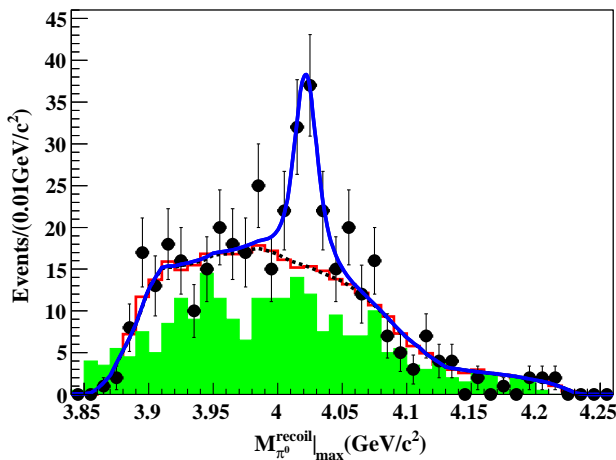
FIG. 2 (color online). Sum of the simultaneous fit to the M_{\pi^0}^{\text{recoil}}|_{\text{max}} distribution at \sqrt{s} = 4.23, 4.26, and 4.36 GeV as described in the text. Dots with error bars are data; the green shaded histogram shows the normalized h_c sideband events; the black dashed curve is the background from the fit; the red histogram shows the result from a phase space MC simulation. The solid blue line shows the total fit.
