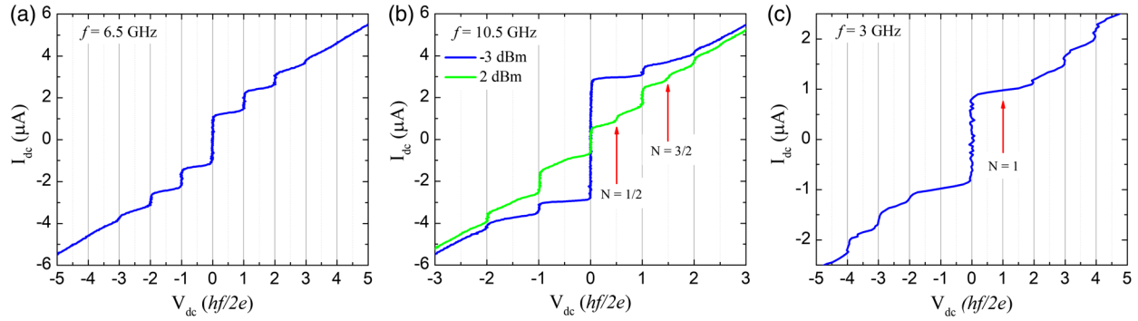
FIG. 3. Observation of the ac Josephson effect in an Al- \text{Cd}_3\text{As}_2 -Al Josephson junction. (a) I - V curves measured with microwave irradiation f = 6.5 GHz for different irradiation power values. Integer Shapiro steps are clearly visible at V_{dc} = Nh f/2e due to the ac Josephson effect. (b) I - V curves measured with microwave irradiation f = 10.5 GHz. Integer Shapiro steps are observed for low irradiation power P = -3 dBm (blue trace). With increasing irradiation power, fractional Shapiro steps emerge. The green trace shows the I - V curve measured with P = 2 dBm. Half-integer Shapiro steps are marked by the red arrows. (c) I - V curves for microwave irradiation of low frequency f = 3 GHz. For high irradiation power, all integer steps are visible. When the power is lowered, step N = 1 is missing, indicating a 4\pi periodic Josephson effect.
