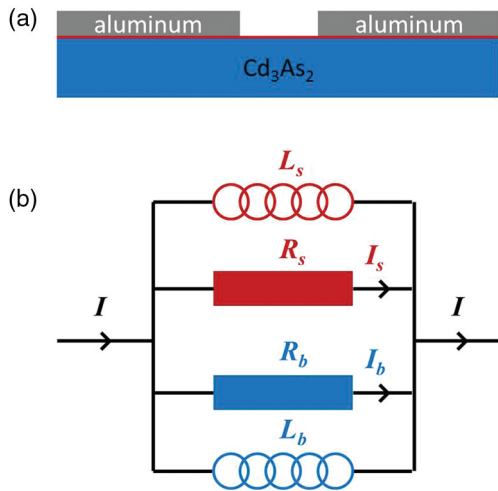
FIG. 4. The SQUID diagram used in our macroscopic model. (a) Schematic sideview of the superconductor- \text{Cd}_3\text{As}_2 -superconductor device structure used in our experiment. (b) Schematic circuit diagram showing the coexistence of bulk-state (indicated by the blue color) and surface-state (indicated by the red color) channels in the Dirac semimetal. L_{s(b)} , R_{s(b)} , and I_{s(b)} are the surface (bulk) inductance, resistance, and current.
