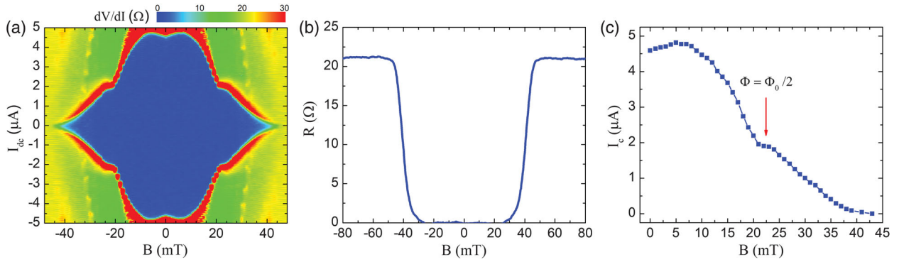
FIG. 2. Current-phase measurements of an Al-Cd 3 As 2 -Al Josephson junction. (a) 2D color plot of dV/dI with respect to the magnetic field and the dc current to better demonstrate the current-phase relationship. The blue area represents the superconducting state and the edge exhibits critical current I_c . (b) The magnetoresistance of junction A measured at 12 mK. The resistance remains zero around B = 0 and starts to increase at B = 30 mT. At B > 40 mT, the superconductivity is completely destroyed and the junction is in the normal state. (c) I_c in junction A is plotted as a function of magnetic field. I_c enhancement induced by the magnetic field has been observed in the low magnetic-field regime due to the strong spin-orbit coupling. The weak minimum at B = 22 mT labeled by the arrow corresponds to \Phi = \Phi_0/2 , indicating a \pi -period supercurrent.
