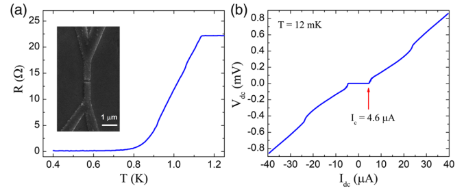
FIG. 1. Experimental configuration and observation of supercurrents in \text{Cd}_3\text{As}_2 . (a) The resistance of a superconductor- \text{Cd}_3\text{As}_2 -superconductor junction versus temperature at zero magnetic field. A zero-resistance state is reached below T_c = 0.8\text{K} . Inset shows a scanning electron microscopy image of a Josephson junction. (b) The current-voltage ( I - V ) characteristic of junction A measured at T = 12\text{mK} . Supercurrent is observed with a critical current I_c = 4.6\mu\text{A} .
