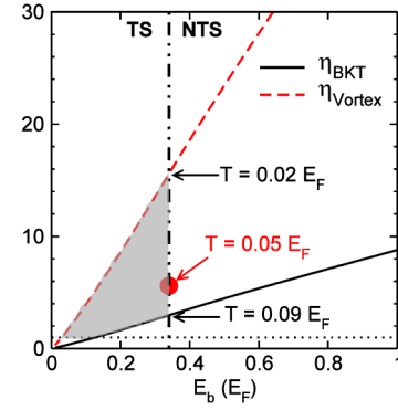
FIG. 3 (color online). (Color online) Plot of \eta = \epsilon_m/T as a function of E_b . h = 0.8E_F and \alpha K_F = 1.6E_F . Dashed-dotted line: E_b^c = 0.33E_F as the corresponding boundary between topological superfluids (TS) and nontopological superfluids (NTS) [see the E_g = T line in Fig. 2(a) for the determination of the phase boundary]. Dotted line: \eta = 1 . Filled circle corresponds to \eta at T = 0.05E_F . The shadow region is the possible parameter region for observing MFs.
